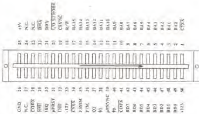
Figure C-9 Expansion connector
